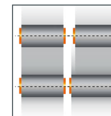
Single-sided drum suspension on the HD 8 and HD 10C models ensures complete compaction right up to the edge.
